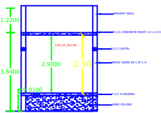
SECTION ON "AA"
