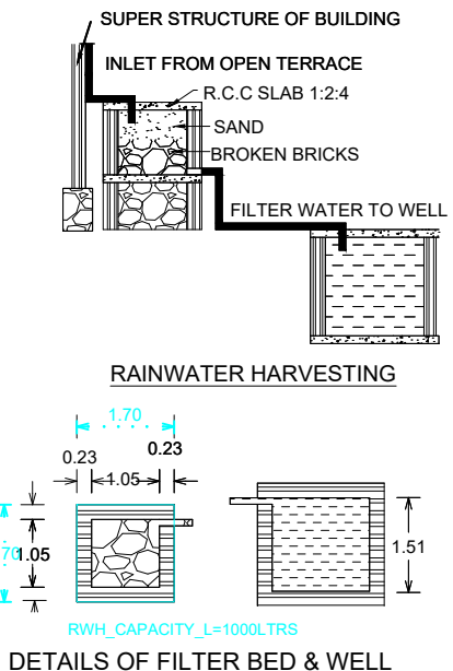
DETAILS OF FILTER BED & WELL
