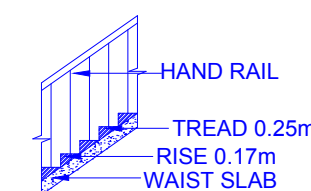
STAIR CASE DETAIL
