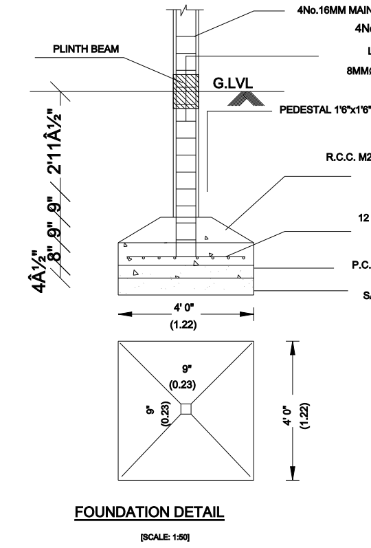
FOUNDATION DETAIL
