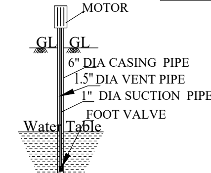
SEC. OF BOREWELL
