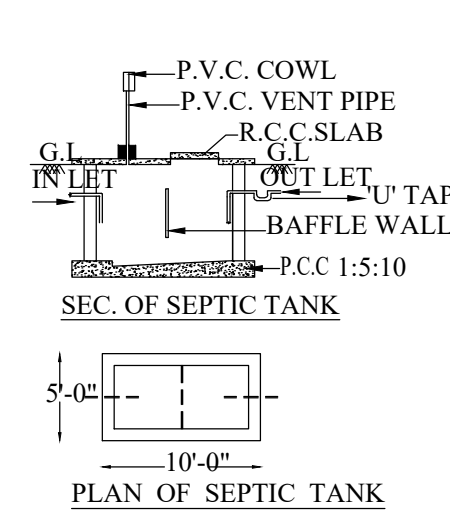
SEC. OF SEPTIC TANK
