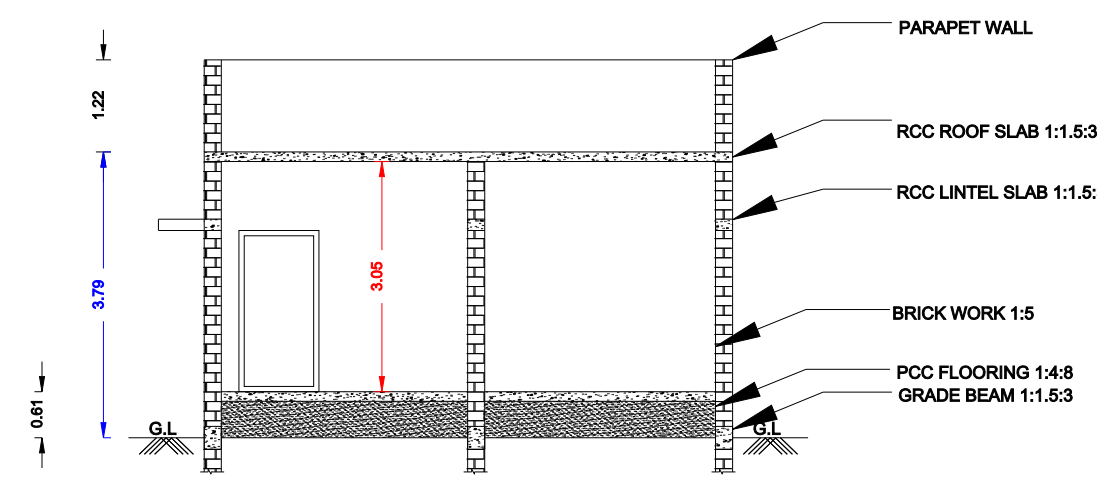
BLOCK#2 SECTION ON 86"AB#6"
