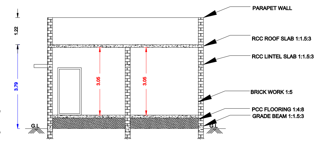
BLOCK#3 SECTION ON 86"AB#6"
