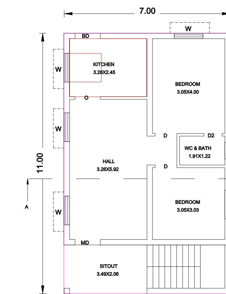
EXI. GROUND FLOOR PLAN 86" BLOCK 2
