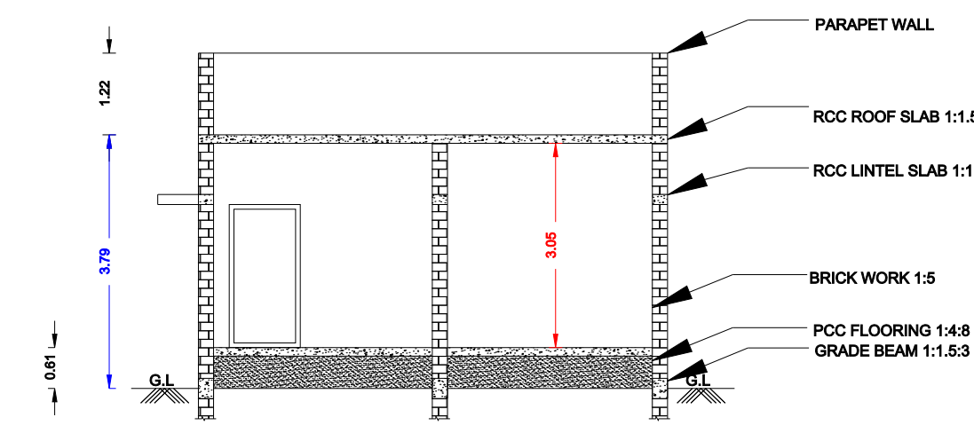
BLOCK#1 SECTION ON 86"AB#6"
