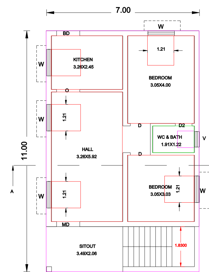
PRO. GROUND FLOOR PLAN 86" BLOCK 3
