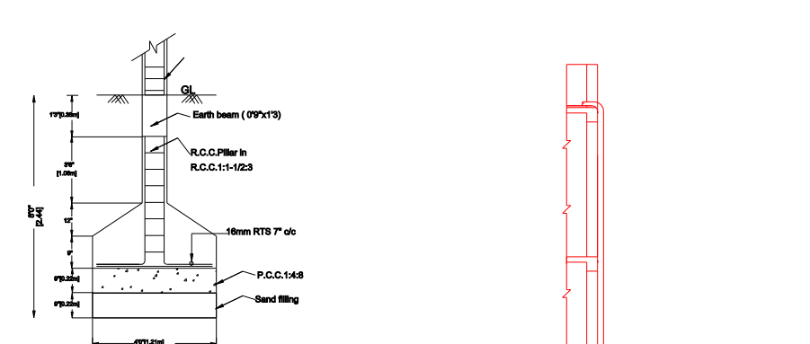
FOUNDATION DETAILS
