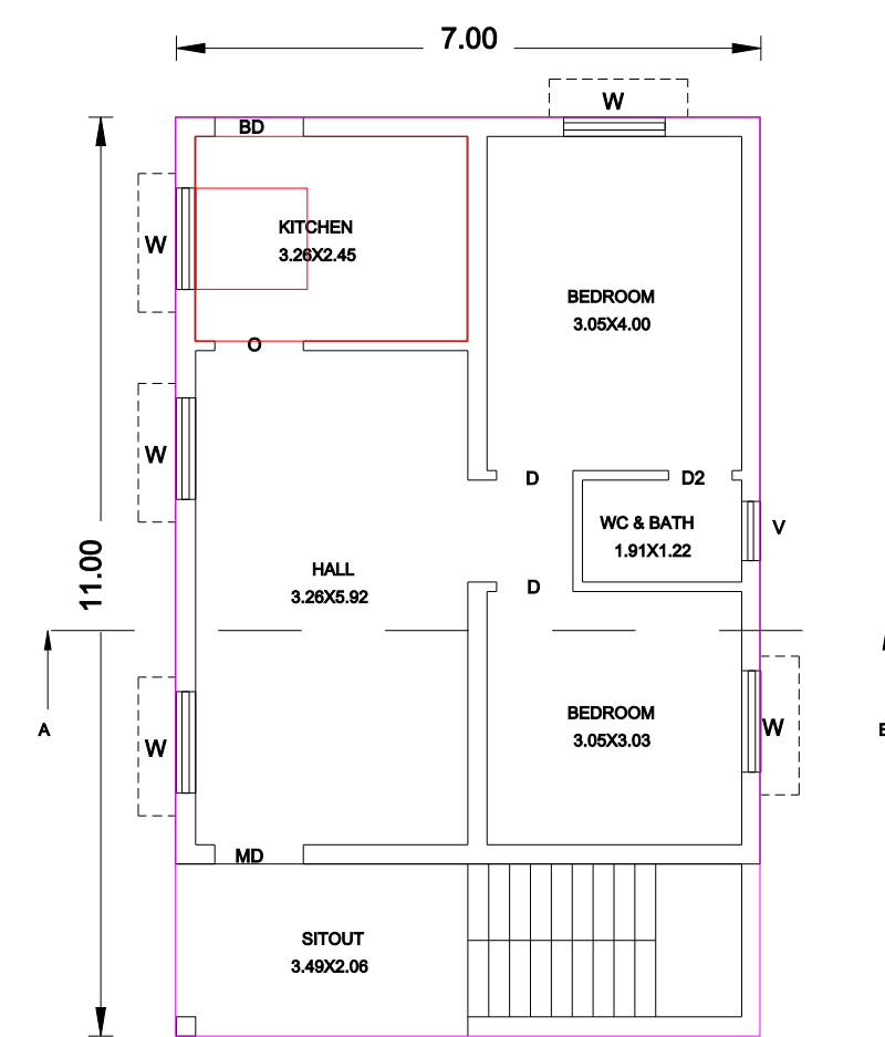
EXI.GROUND FLOOR PLAN 86" BLOCK 1
