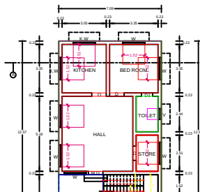
SUPER STRUCTURE OF BUILDING
