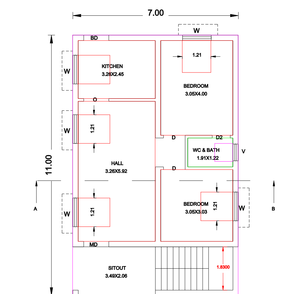
PRO. GROUND FLOOR PLAN 86° BLOCK 1
