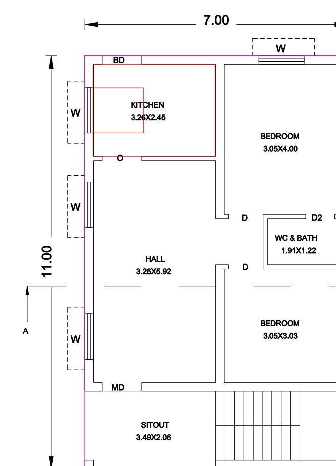
EXI. GROUND FLOOR PLAN 86° BLOCK 2
