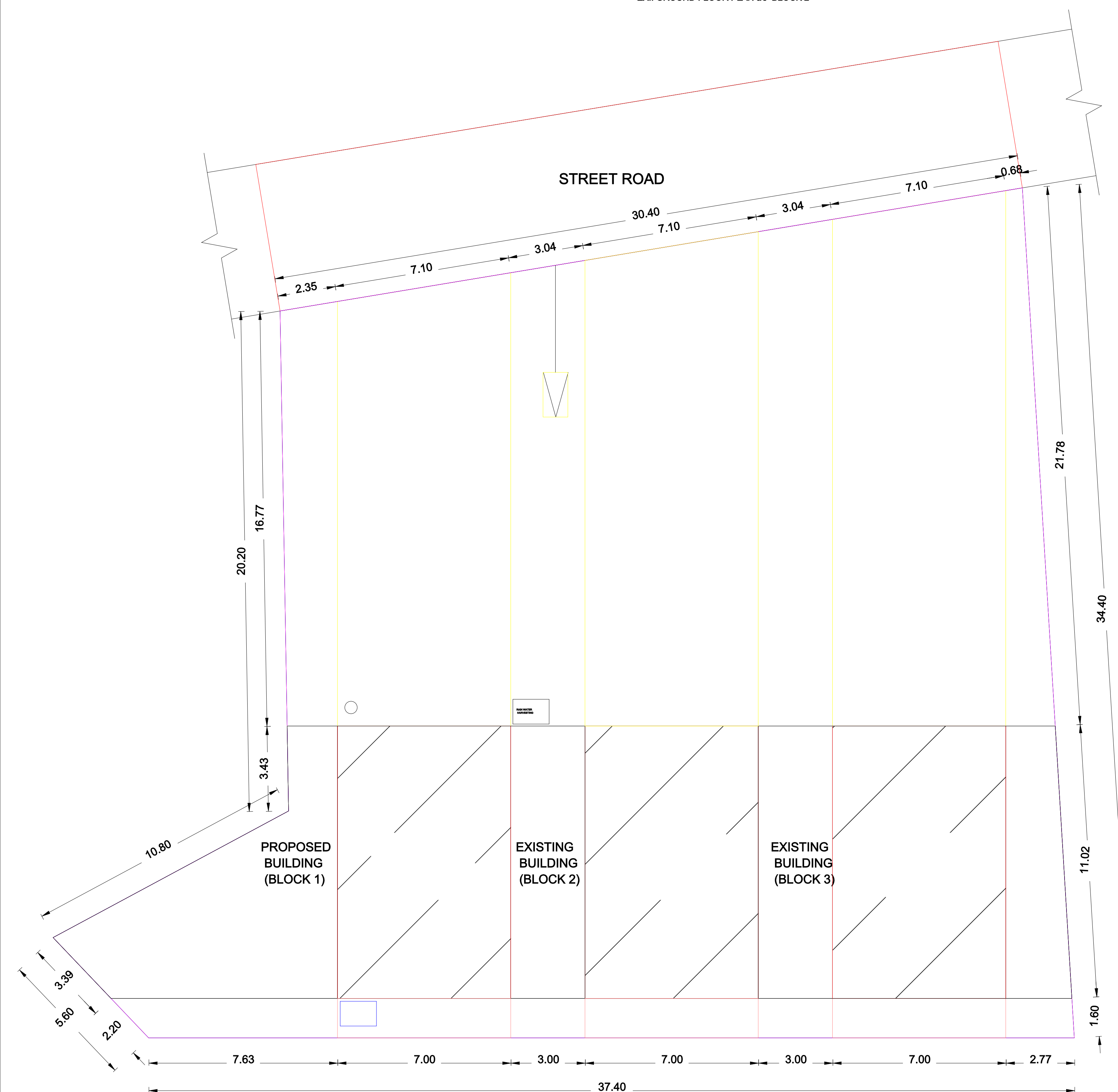
PRO. GROUND FLOOR PLAN 86° BLOCK 1
