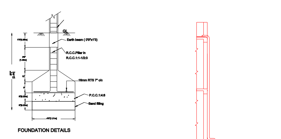
FOUNDATION DETAILS
