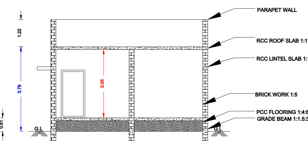
BLOCK#2 SECTION ON 86°AB#6™
