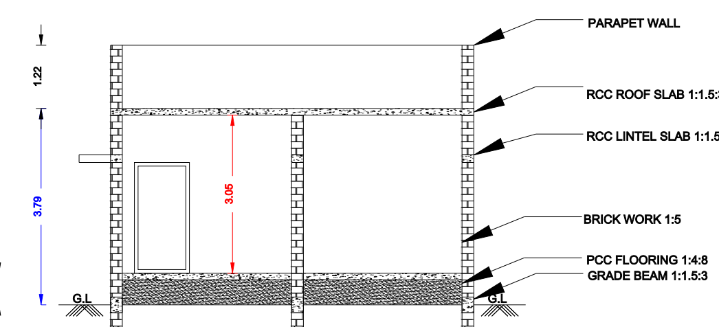
BLOCK#3 SECTION ON 86°AB#6™
