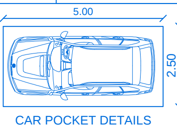
CAR POCKET DETAILS
