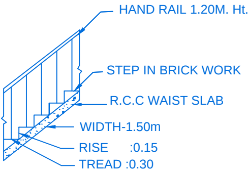
STAIR DETAIL
