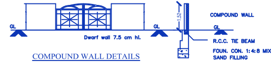
COMPOUND WALL DETAILS
