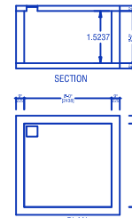
DETAILS OF COLLECTION SUMP FOR RAIN WATER HARVESTING OF ROOF TOP RAIN WATER RWH_CAPACITY_L=5000LTRS
