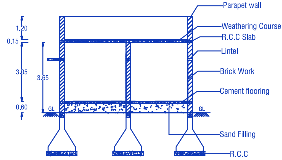
CROSS SECTION ON 'AB'
