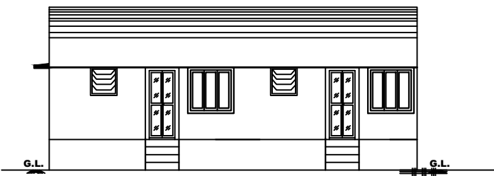
FRONT ELEVATION
