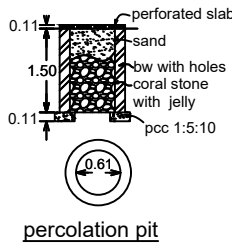
percolation pit
