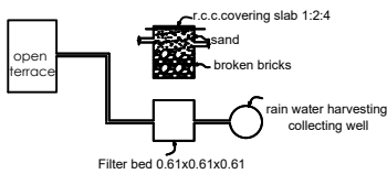
DETAILS OF RAIN WATER HARVESTING SYSTEM
