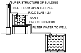
RAINWATER HARVESTING
