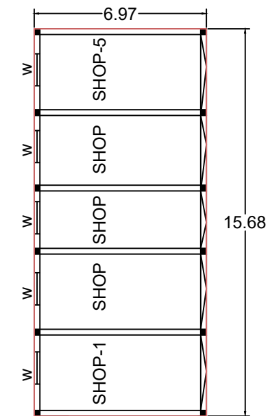
EXISTING BUILDING
