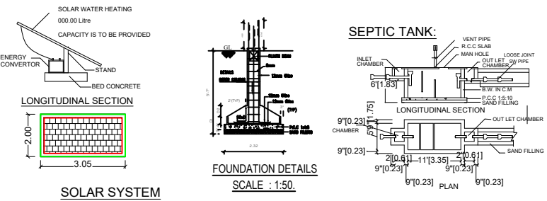
SOLAR SYSTEM
