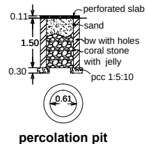
percolation pit
