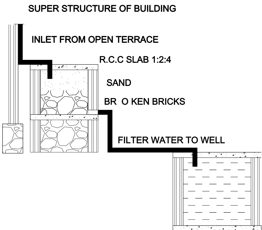
RAINWATER HARVESTING
