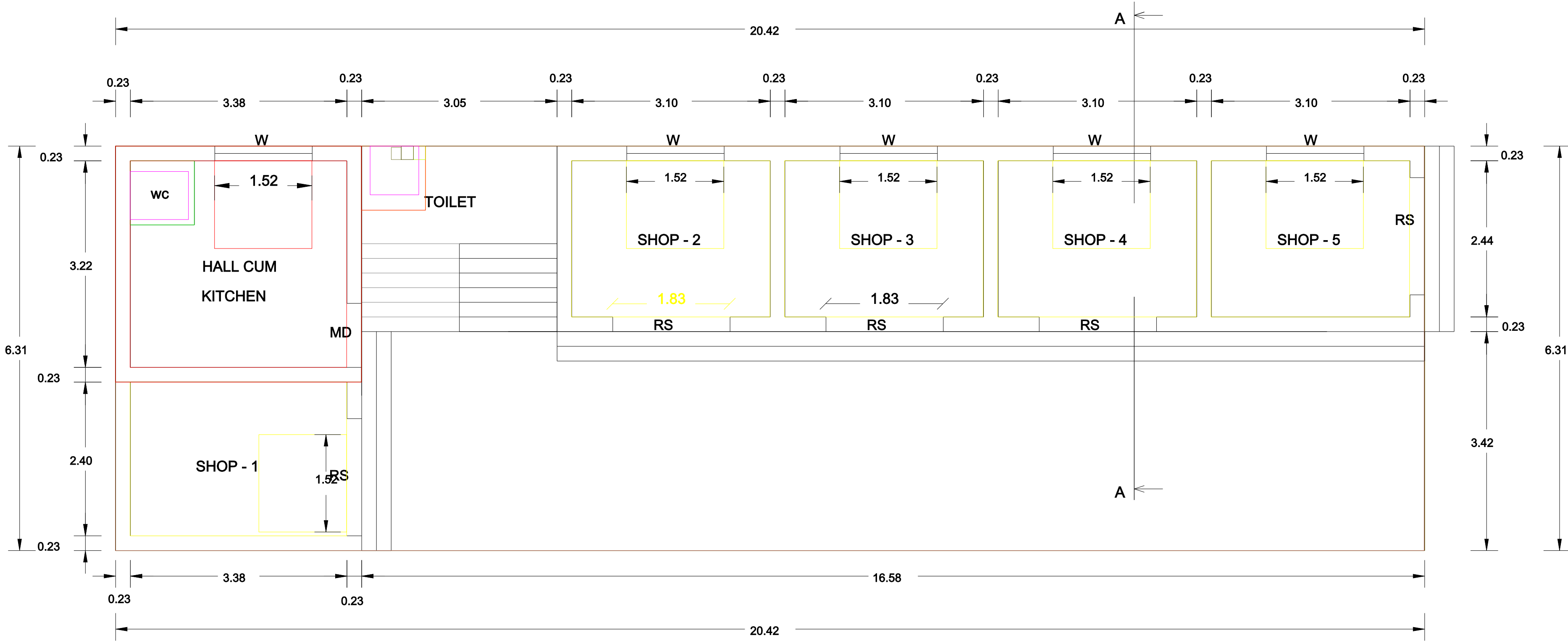
PLAN
