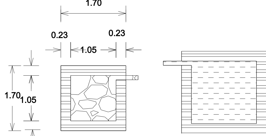
DETAILS OF FILTER BED & WELL
