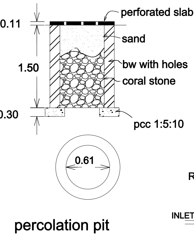
percolation pit
