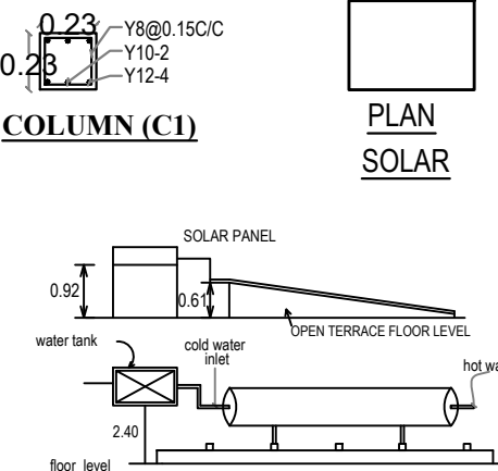
Details of solar water heating system
