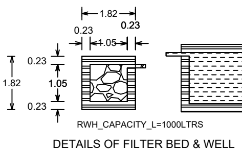
DETAILS OF FILTER BED & WELL
