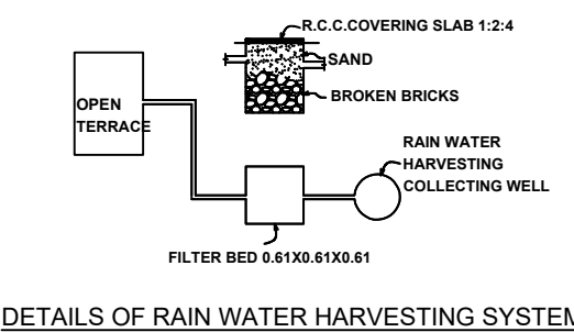
DETAILS OF RAIN WATER HARVESTING SYSTEM
