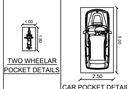
CAR POCKET DETAILS
