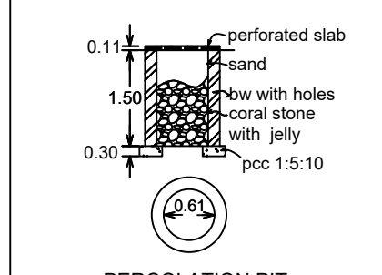
PERCOLATION PIT
