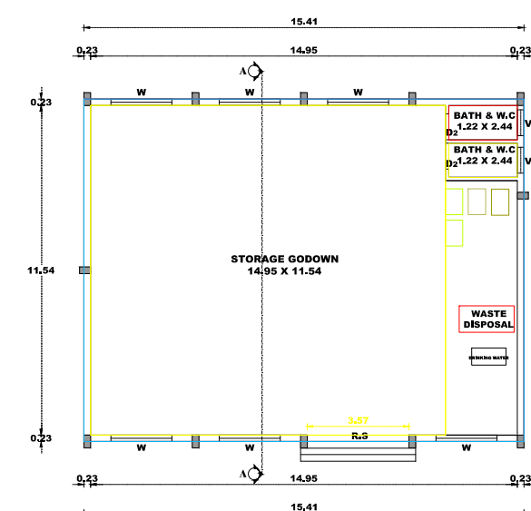
GROUND FLOOR PLAN ( BLOCK - I )
