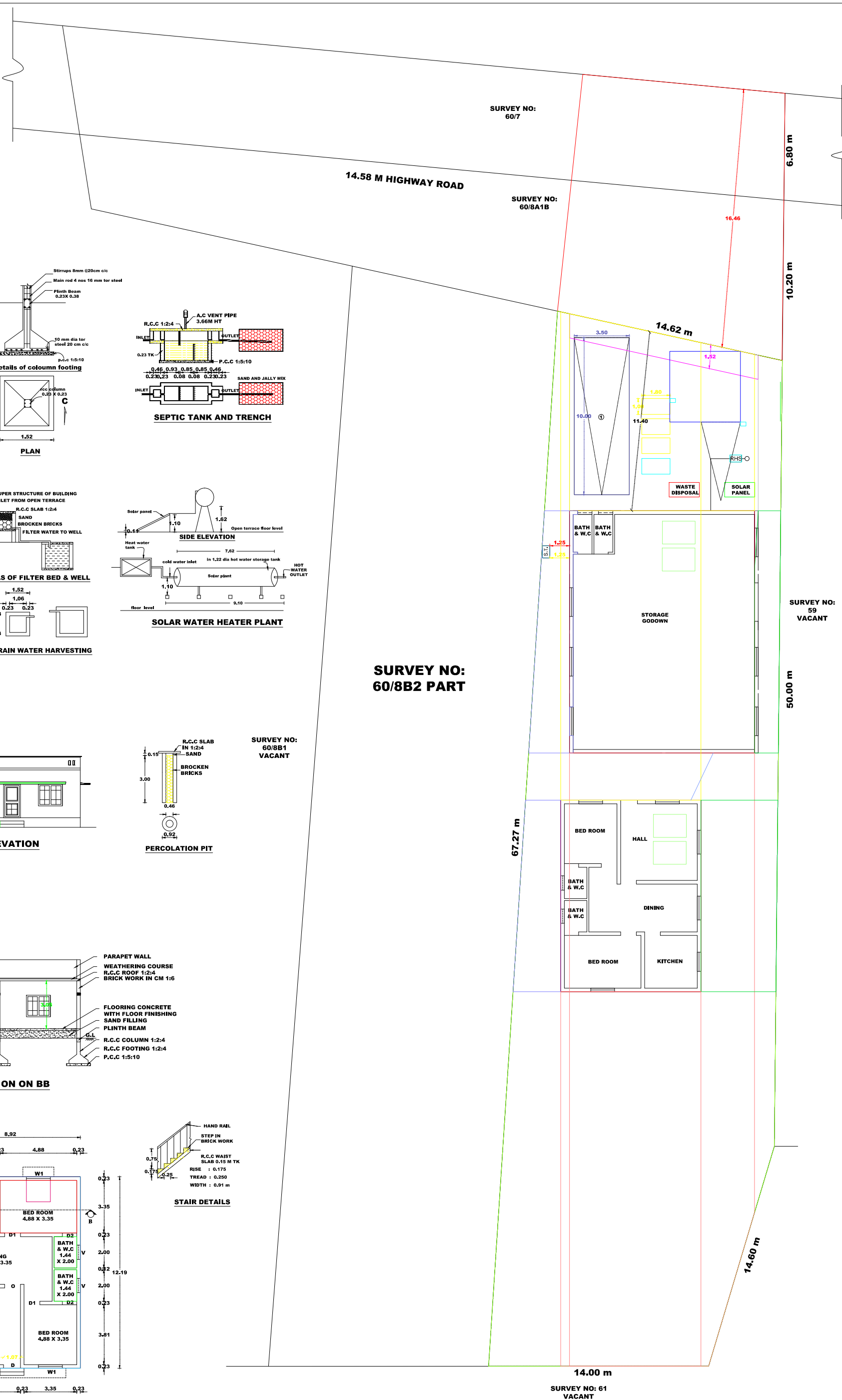
GROUND FLOOR PLAN ( BLOCK - II )
