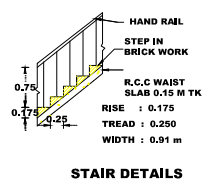
STAIR DETAILS
