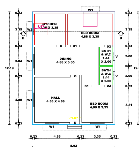
GROUND FLOOR PLAN ( BLOCK - II )
