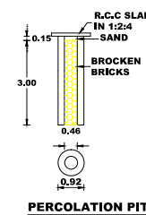
PERCOLATION PIT
