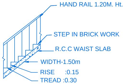
STAIR DETAIL
