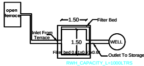
Plan Of Filter Bed & Well
