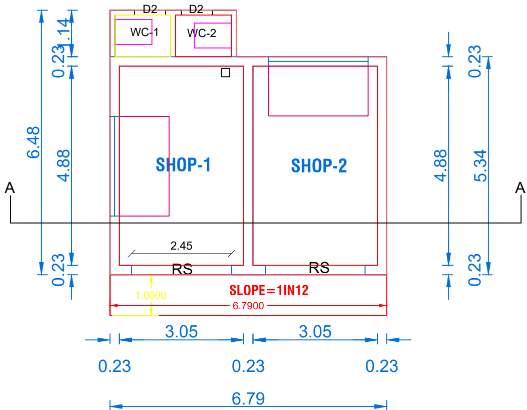
PRO GROUND FLOOR
