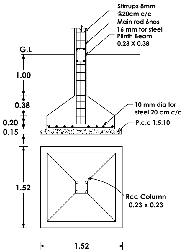
DETAILS OF COLUMN FOOTING
