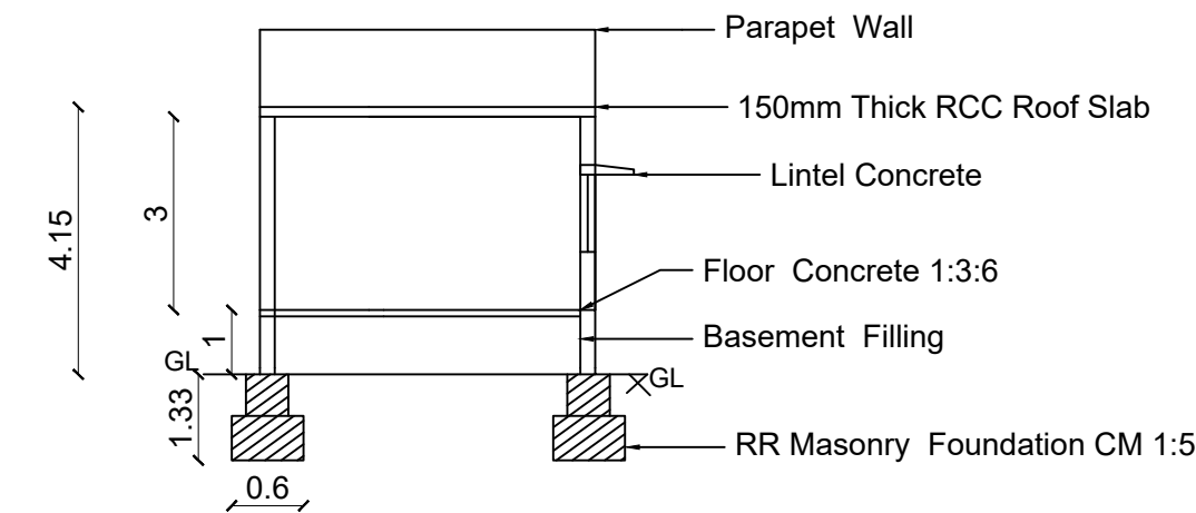
SECTION A - A VIEW
