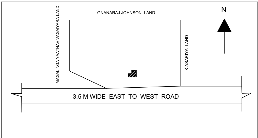
TOPO PLAN
