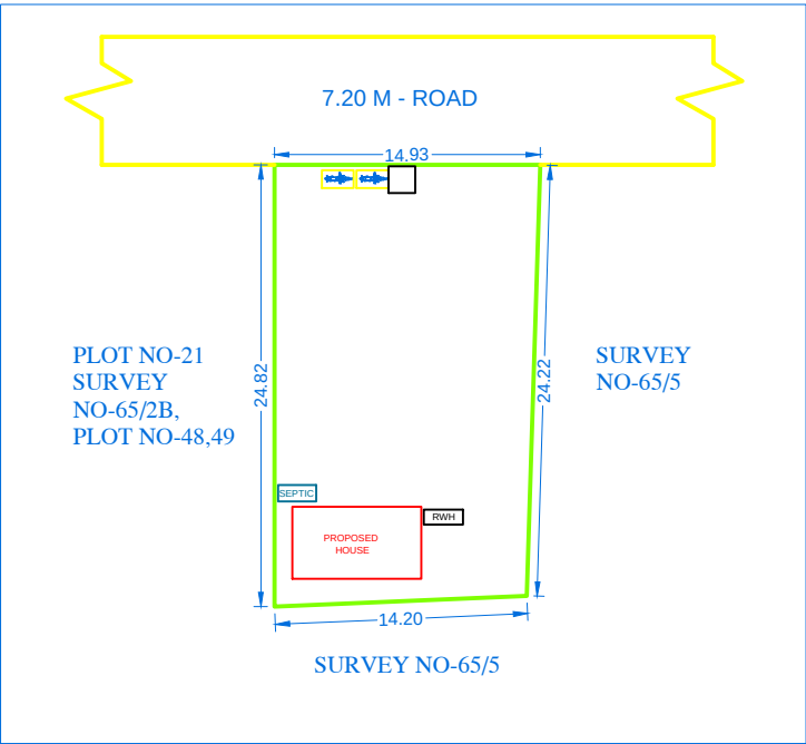
LOCATION PLAN Scale 1:400
