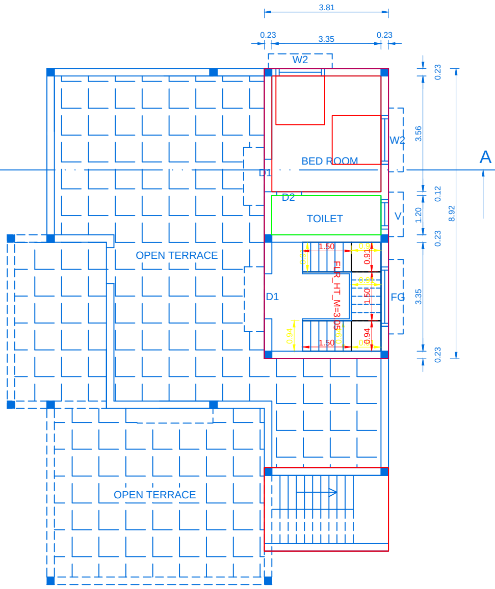
PROP.SECOND FLOOR PLAN
