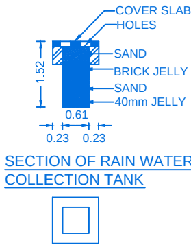
SECTION OF RAIN WATER COLLECTION TANK
