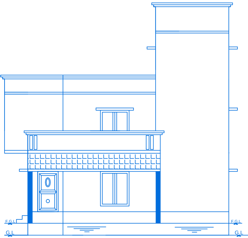
FRONT ELEVATION
