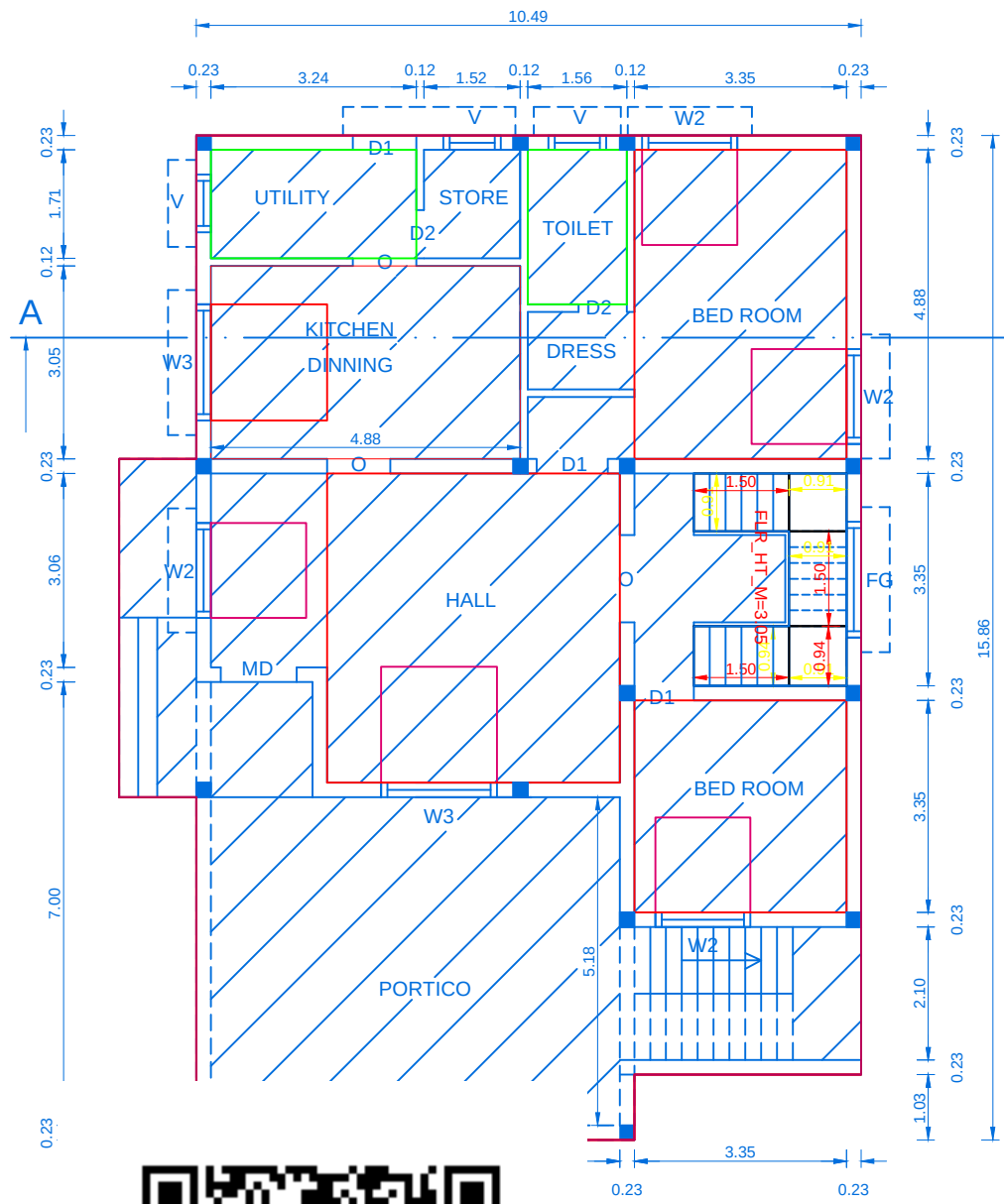
FLOOR PLAN
