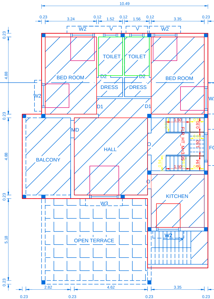
EXG.FIRST FLOOR PLAN
