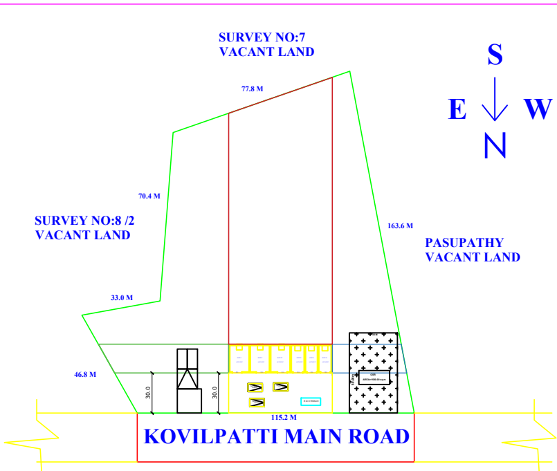
SITE PLAN
