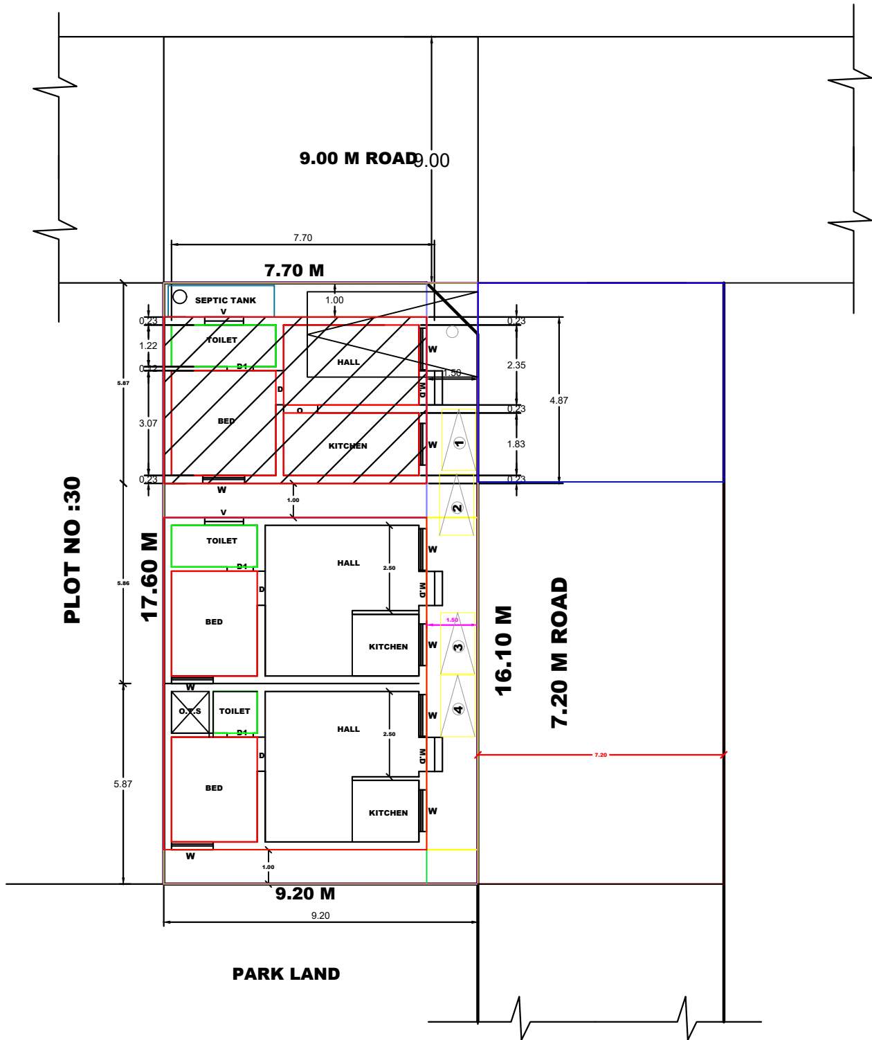
KEY PLAN
