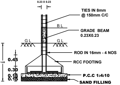
RCC COLUMN DETAILS
