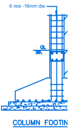
COLUMN FOOTIN
