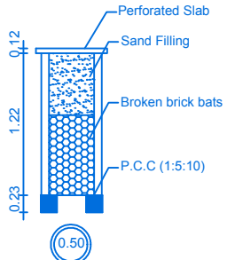
RAIN WATER COLLECTION WELL
