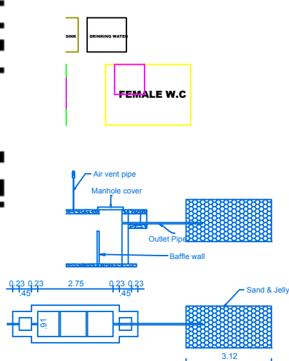
SEPTIC TANK & TRENCH
