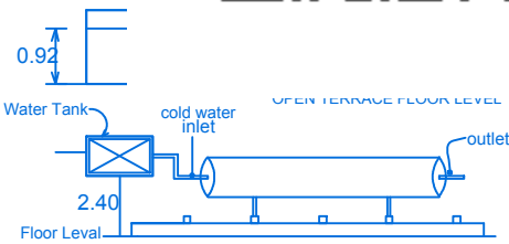
Details of solar water heating system
