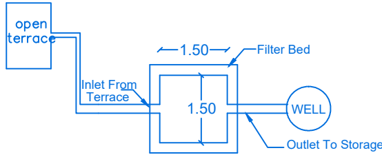
Plan Of Filter Bed & Well
