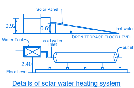
Details of solar water heating system
