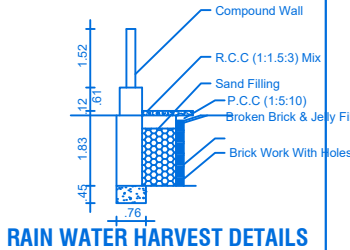
RAIN WATER HARVEST DETAILS
