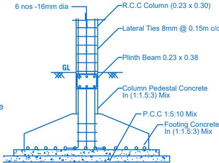
COLUMN FOOTING DETAILS
