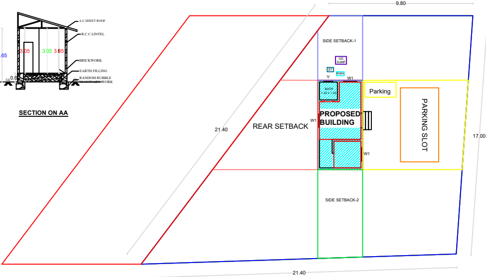
RESIDUARY PLOT SKETCH, SUPER IMPOSED SKETCH (SITE PLAN)
