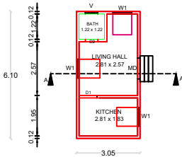
PROPOSED GROUND FLOOR PL
