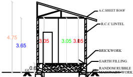
SECTION ON AA
