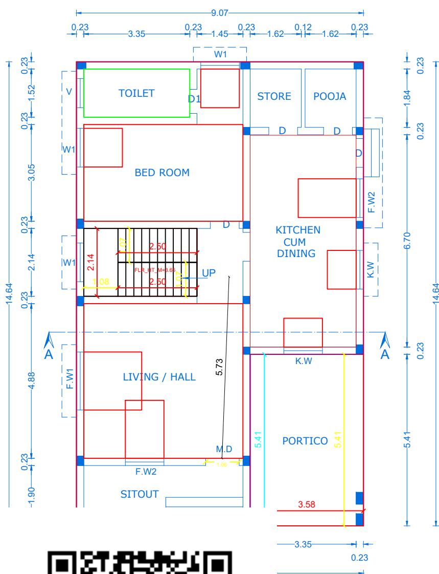
PLAN
