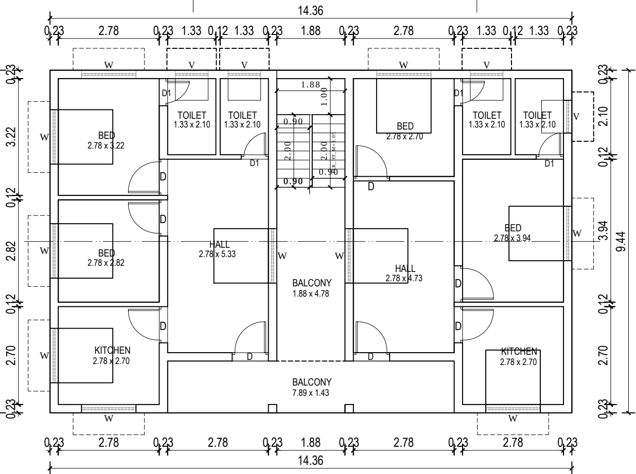
PRO.FF PLAN
