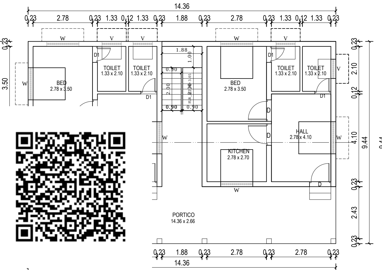
PRO.GF PLAN
