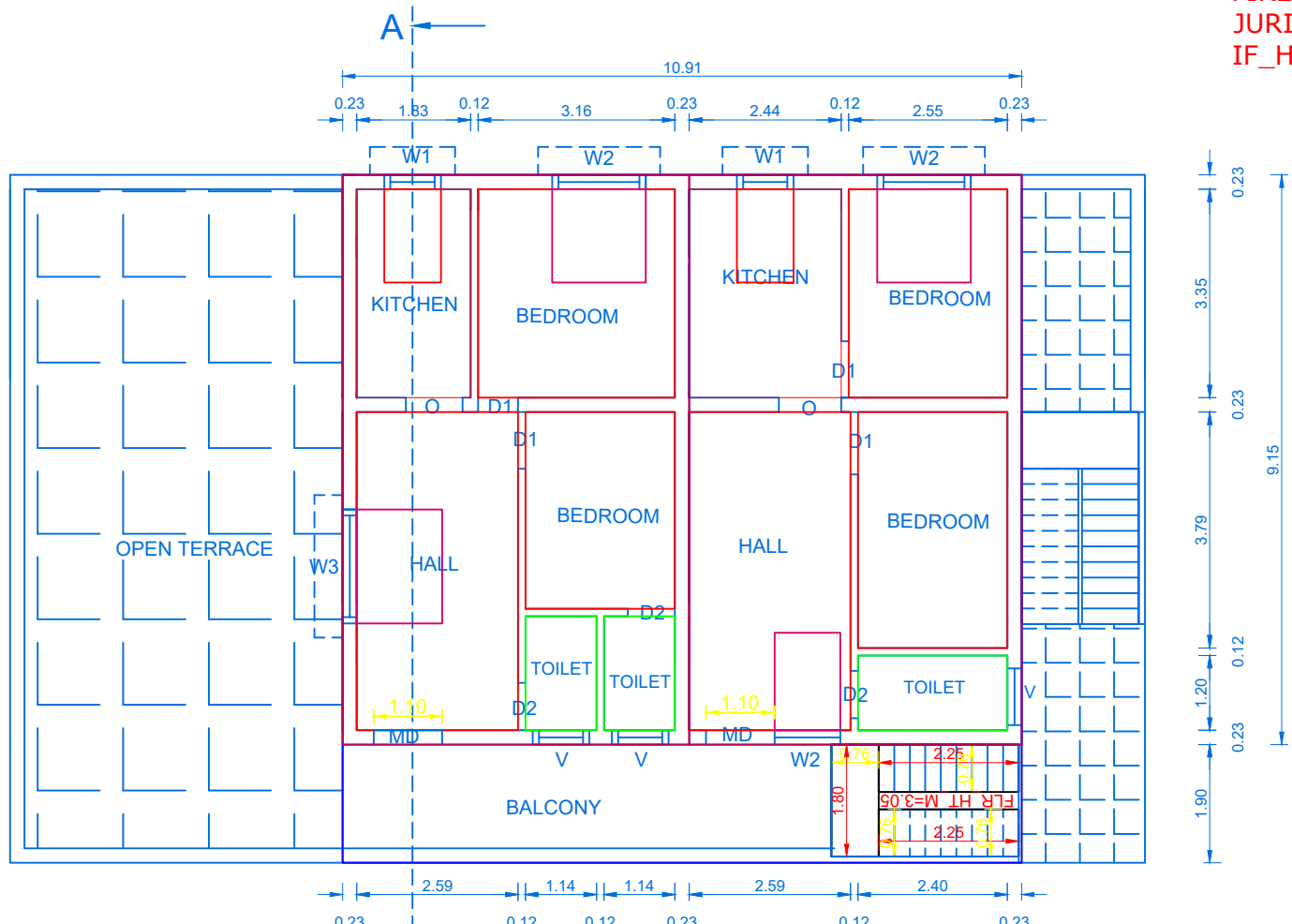
PROP.FIRST FLOOR PLAN
