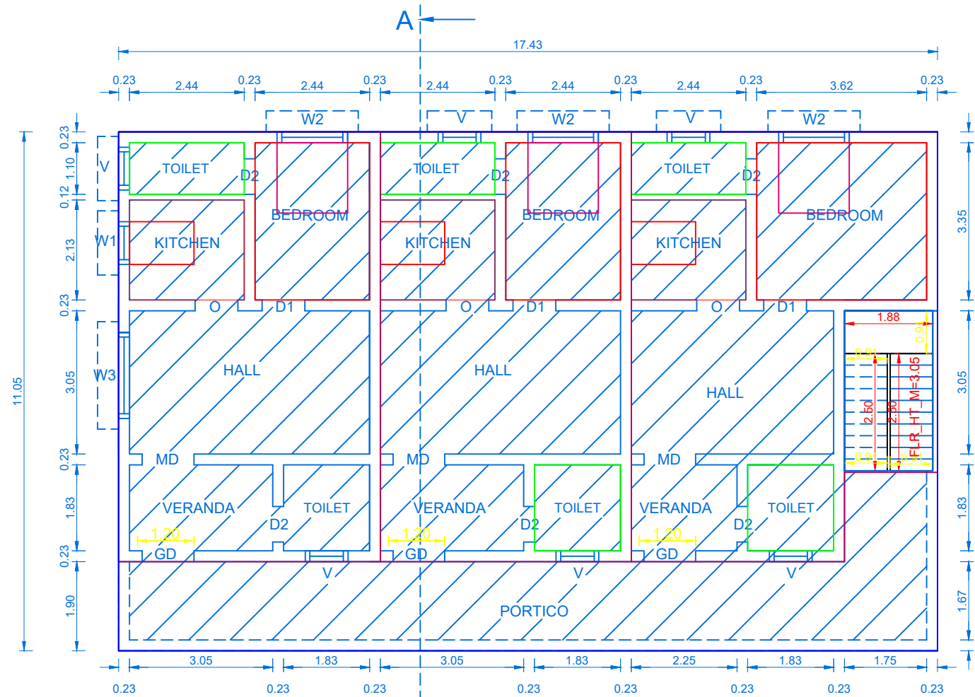
EXG.GROUND FLOOR PLAN
