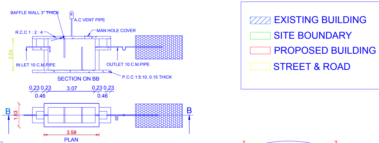
SEPTIC TANK AND TRENCH & U TRAP ADOPTED
