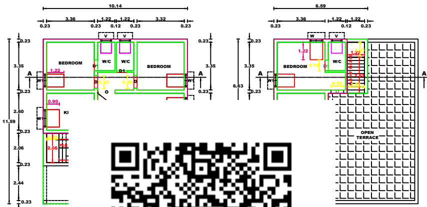
FLOOR PLAN
