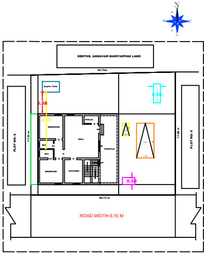
LOCATION PLAN
