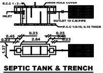
SEPTIC TANK & TRENCH
