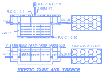
SEPTIC TANK AND TRENCH
