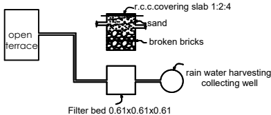
DETAILS OF RAIN WATER HARVESTING SYSTEM
