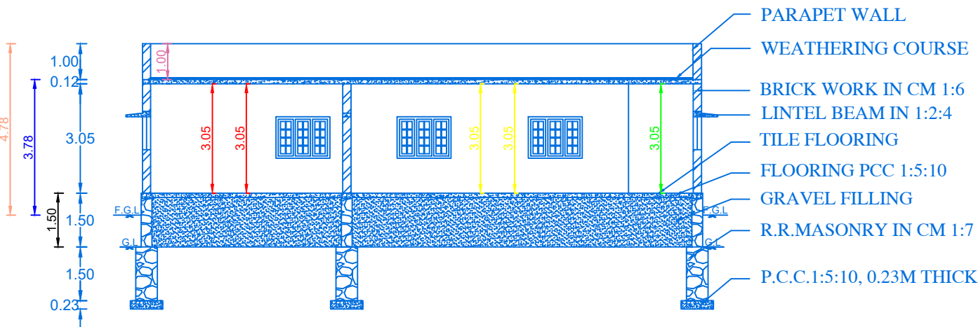
SECTION ON "V-B"
