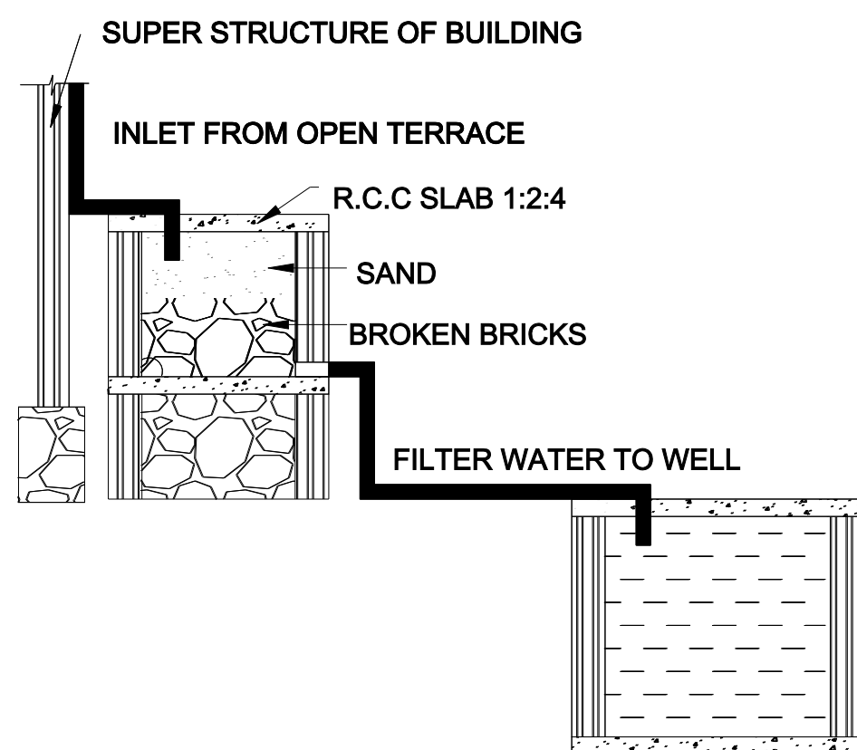
RAINWATER HARVESTING
