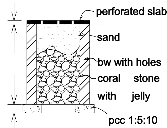
percolation pit
