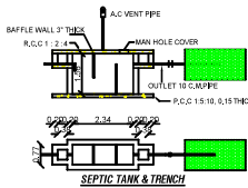
SEPTIC TANK & TRENCH
