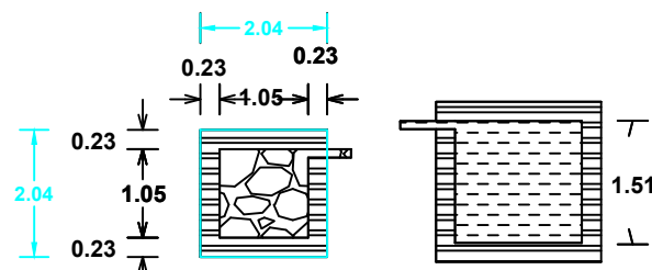
DETAILS OF FILTER BED & WELL
