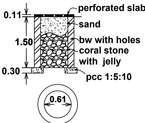
percolation pit
