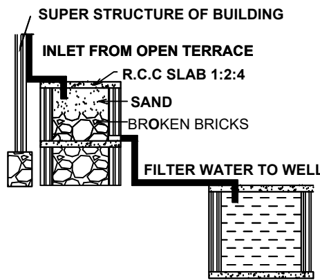
RAINWATER HARVESTING
