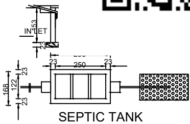
SEPTIC TANK
