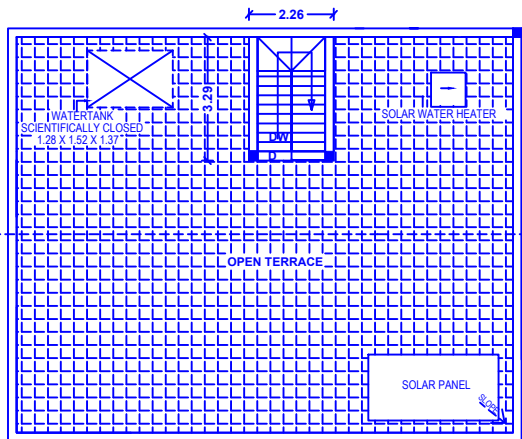
PROPOSED TERRACE PLAN
