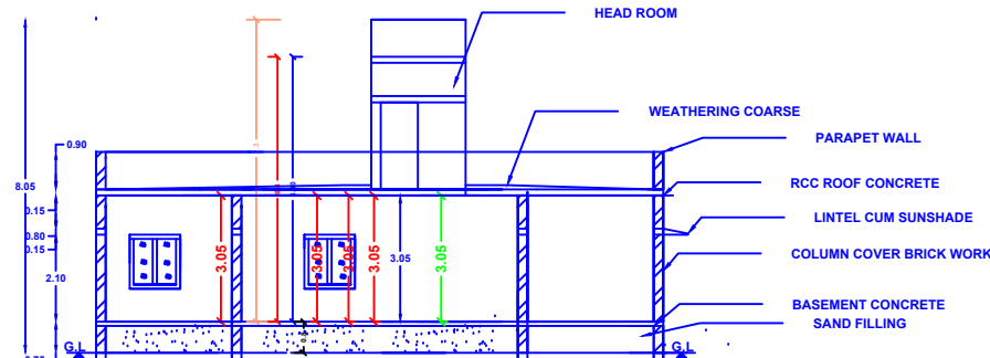
SECTION AB
