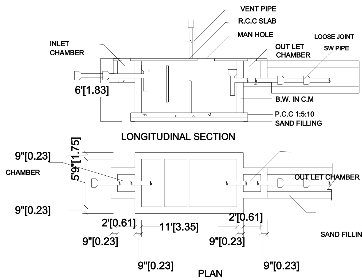
SEPTIC TANK:
