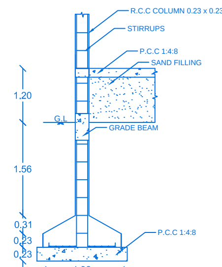
COLUMN DETAIL (SCALE 1:50)
