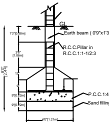
FOUNDATION DETAILS
