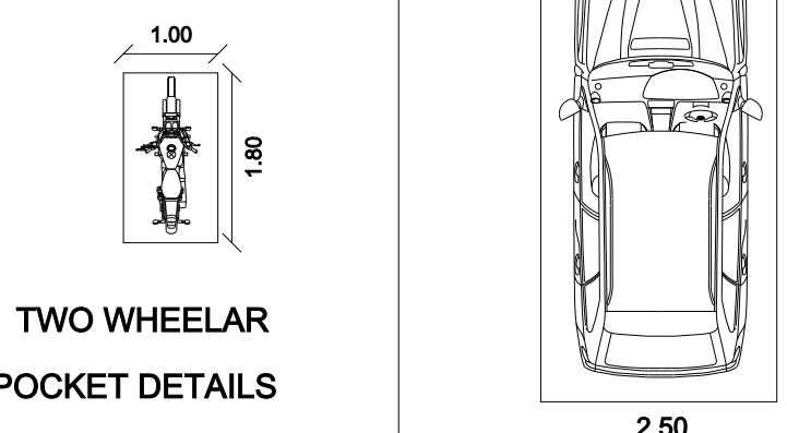
CAR POCKET DETAILS
