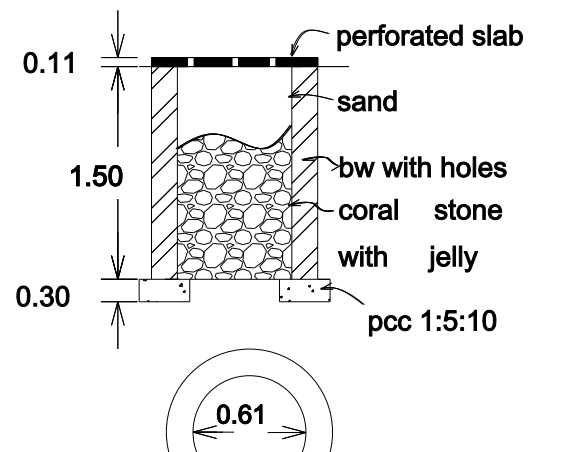
PERCOLATION PIT
