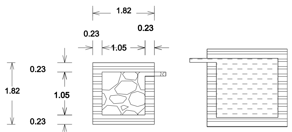
DETAILS OF FILTER BED & WELL
