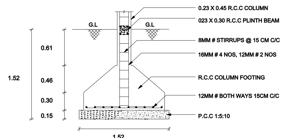
COLUMN FOOTING DETAILS
