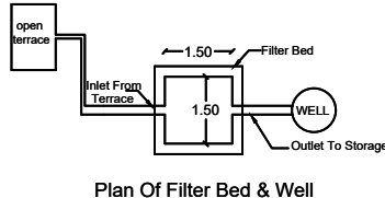
Plan Of Filter Bed & Well
