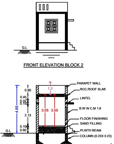
CROSS SECTION VIEW AB BLOCK 2
