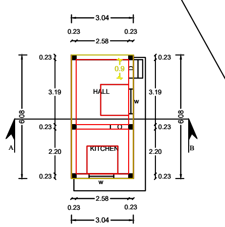
GROUND FLOOR BLOCK 2
