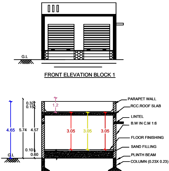
CROSS SECTION VIEW AB BLOCK 1
