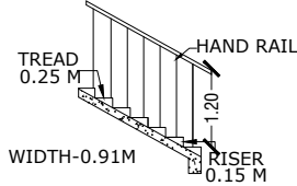
STAIRCASE DETAILS
