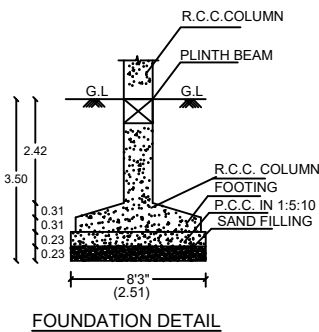
FOUNDATION DETAIL
