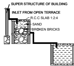
RAINWATER HARVESTING
