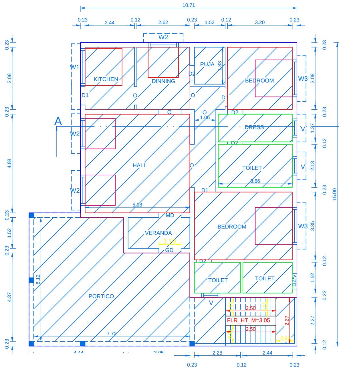
FLOOR PLAN
