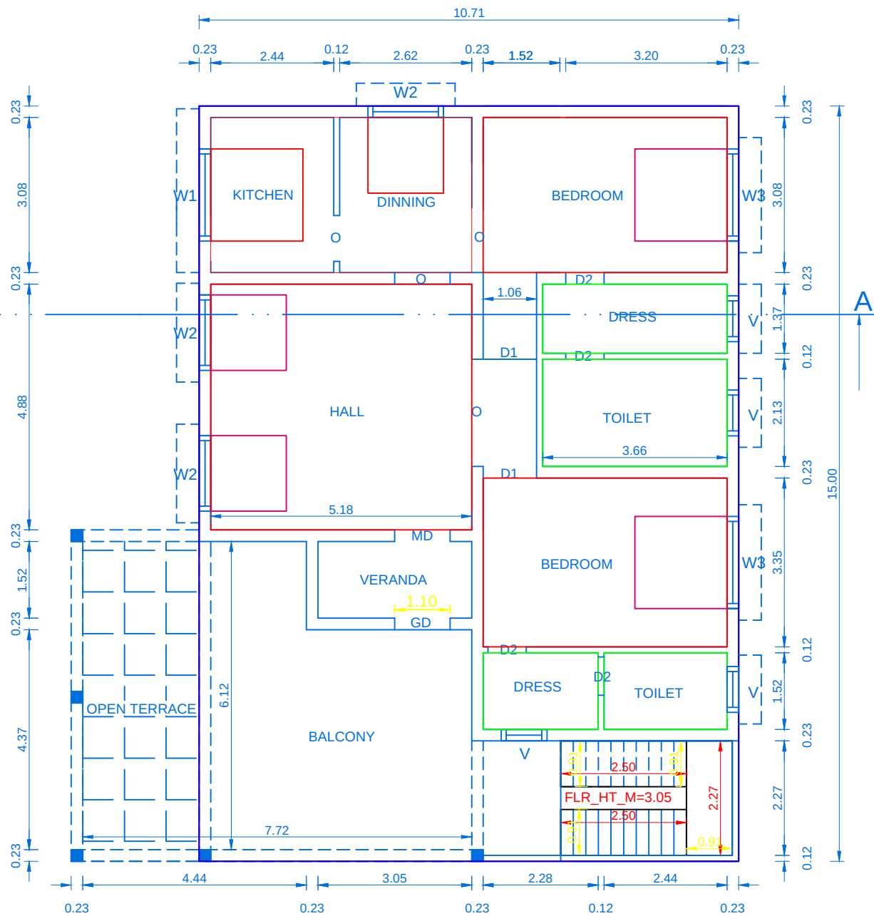
PROP.FIRST FLOOR PLAN
