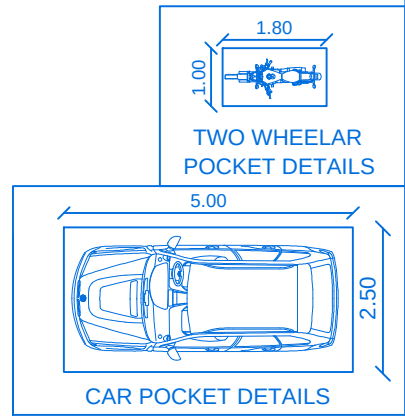
CAR POCKET DETAILS
