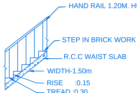
STAIR DETAIL
