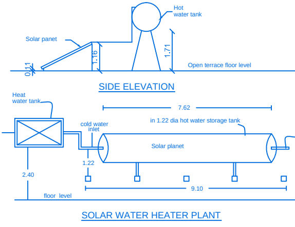
SOLAR WATER HEATER PLANT
